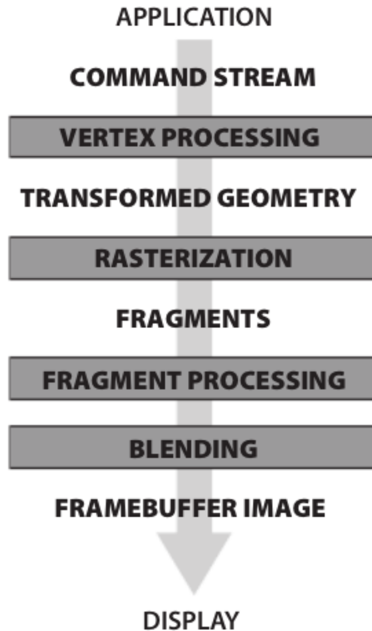
Figure 8.1. The stages of a graphics pipeline.
