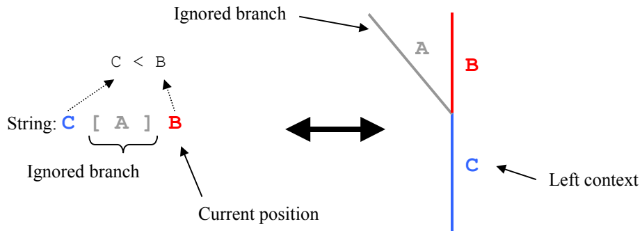
Figure 7 Matching left context, lateral branches implicitly ignored
