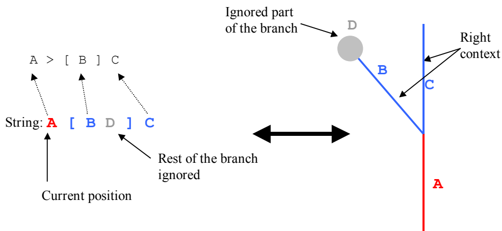
Figure 3 Matching right context, remainder of lateral branch is implicitly ignored
